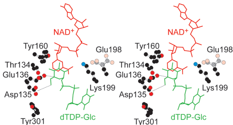
FIGURE 2: Stereoview of a 4,6-dehydratase/ \text{NAD}^+ /dTDP-glucose active site model. The dTDP-glucose was placed in the 4,6-dehydratase active site (PDB file 1BXK) using structural alignments with the UDP-galactose-4-epimerase UDP-glucose abortive complex (1XEL, 23) as a guide; no energy minimization was performed. The approximate placement of the glucopyranose moiety is constrained by the requirement for hydride transfer from C4 to \text{NAD}^+ , and from NADH back to C6. These constraints may necessitate a slightly different active site conformation, or a conformation change during chemistry, but Asp135 and Glu136 will always be adjacent to C6(OH), and Glu198 and Lys199 will be closer to C2(OH) and the pyrophosphate moiety. Ambiguities in the placement of the Glu198 side chain in the 4,6-dehydratase/ \text{NAD}^+ structure are represented by two overlapping ball-and-stick models, and indicated by lighter coloration. The stereoview was generated using Molview and PDB files 1XEL and 1BXK (23, 24).
